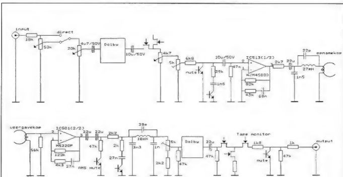
Philips DCC 900
